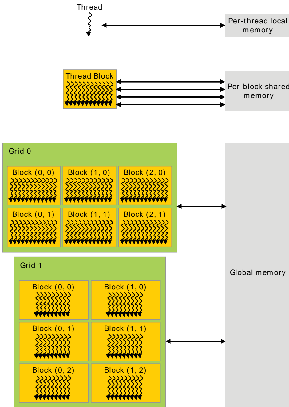
Figure 7 Memory Hierarchy
